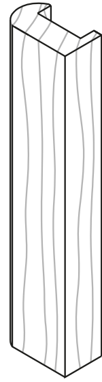
m2 28x16 mm. reb 19x5 mm.
