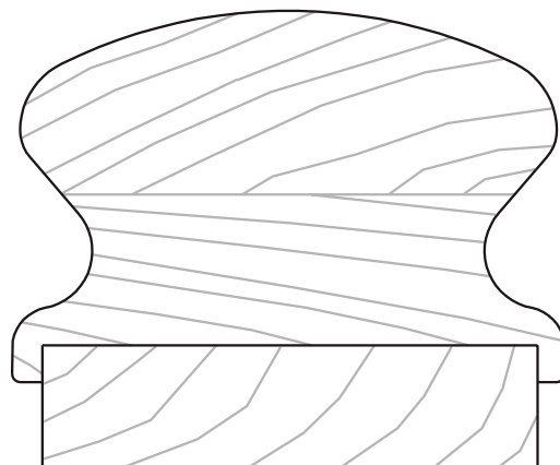
756C (70x45 mm. tabla 60x15 mm.)
